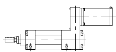
Reverse Parallel Mounting Positions (as viewed from the shaft end)
